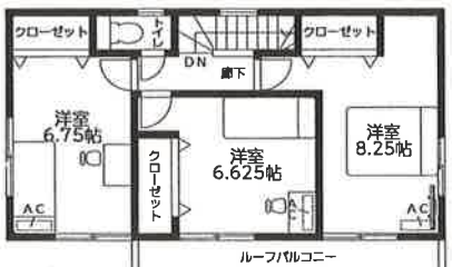
2階平面図:47.83㎡
