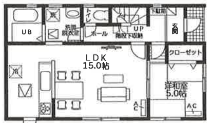
1階平面図:50.52㎡
