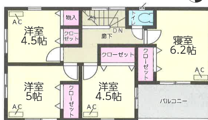
2階平面図:53.46㎡
