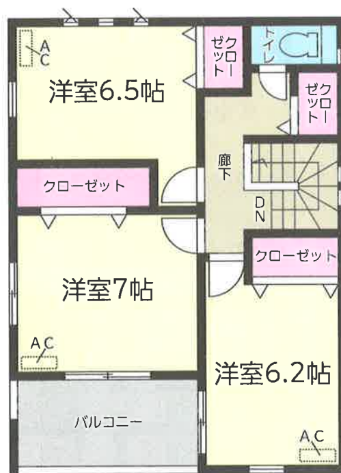
2階平面図:53.86㎡
