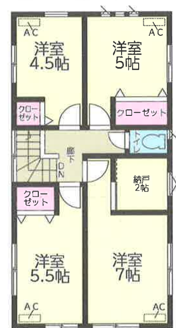
2階平面図:49.00㎡
