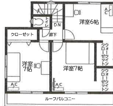
2階平面図:45.96㎡
