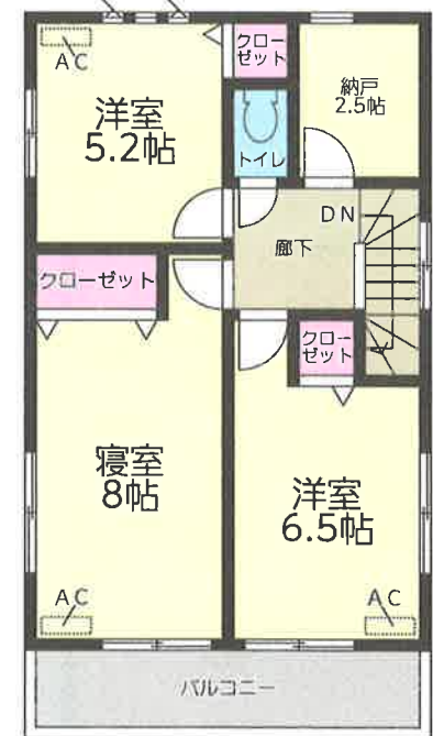
2階平面図:46.17㎡
