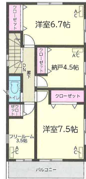
2階平面図:49.00㎡
