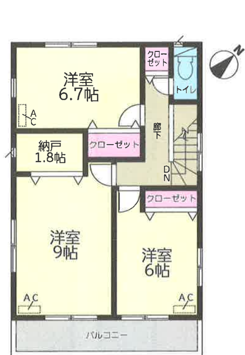
2階平面図: 50.01㎡
