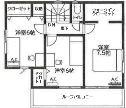
2階平面図:45.96㎡
