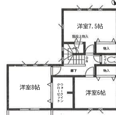
2階平面図:53.82m 2
