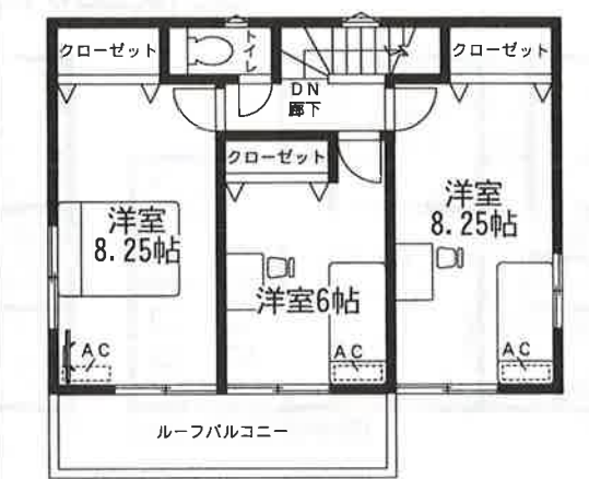
2階平面図:48.45㎡
