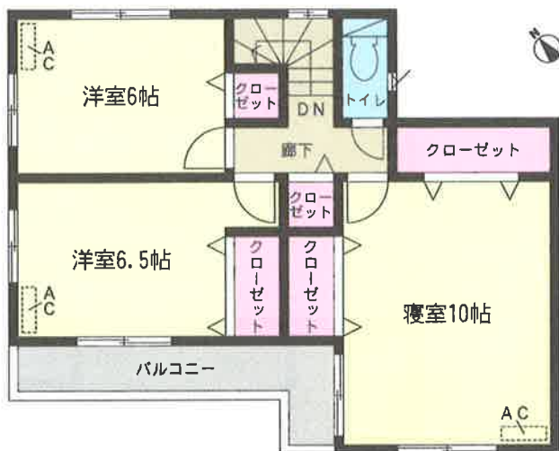
2階平面図:50.22㎡
