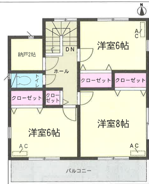
2階平面図:50.22㎡
