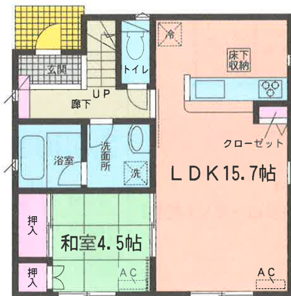
1階平面図:50.22㎡
