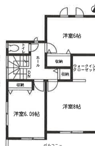
2階平面図:48.45㎡
